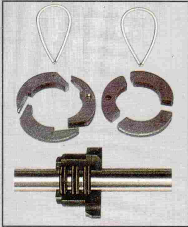
Full floating, self adjusting packing rings
