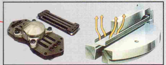
Rectangular, patented, air-cushioned channel valve with free air unloader
