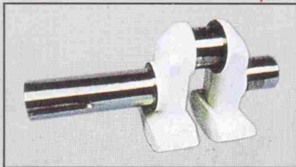
Die forged balanced crankshaft, with rifle drilled oil passage
