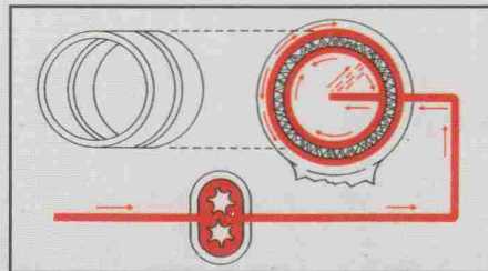
Bearings float in pressurized oil layers. Oil circulated by an internal gear pump driven through a pin attached to crankshaft
